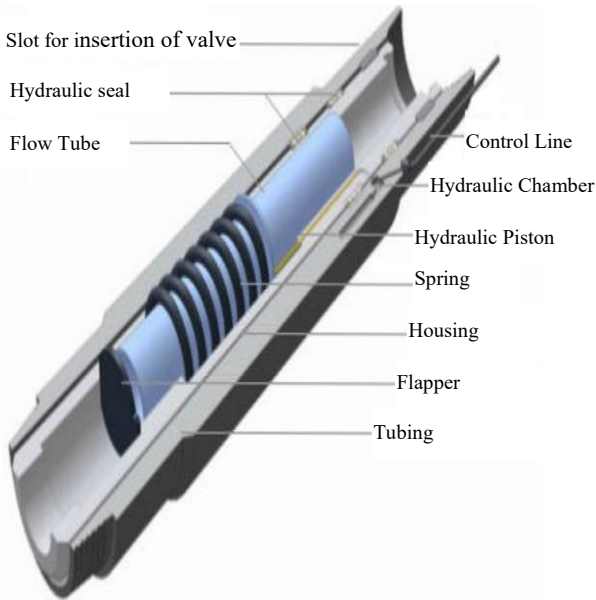
Fig. 3 Schematic drawing of DHSV
