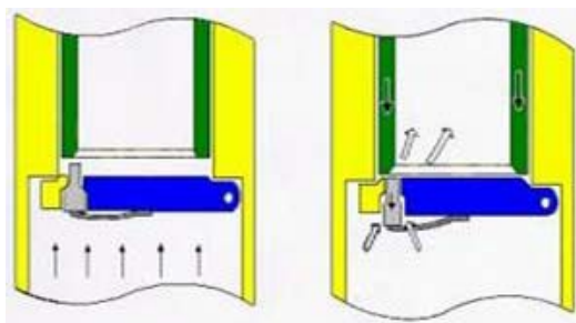
Fig. 7 Self-equalization mechanism
