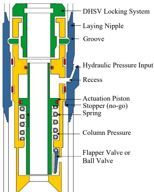
Fig. 6 Schematic drawing of retrievable DHSV
