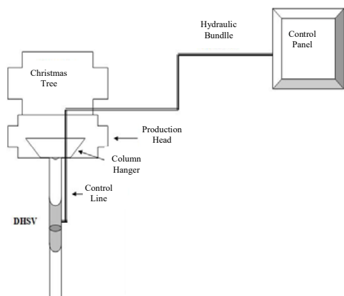
Fig. 1 Schematic drawing of the DHSV circuit
