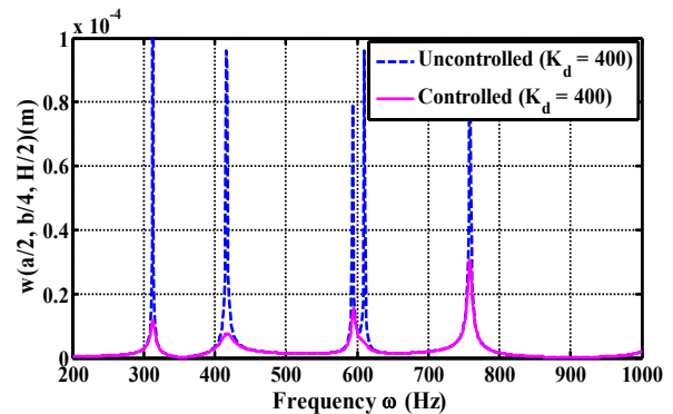
Fig. 6 Frequency response functions for the transverse displacement w(a/2, b/4, H/2) of a clamped-clamped P/M/P multiferroic doubly curved shell with patches at the edges ( a = 200H, R_1=10a; R_2=10R_1 )
