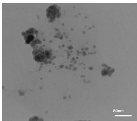
Fig. 7 TEM image of the green synthesized Ag_3PO_4 nanoparticles
