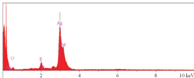
Fig. 6 EDS analysis of Ag_3PO_4 nanoparticles
