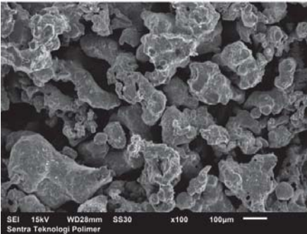
Fig. 5 SEM Visualization of Sintered Copper
