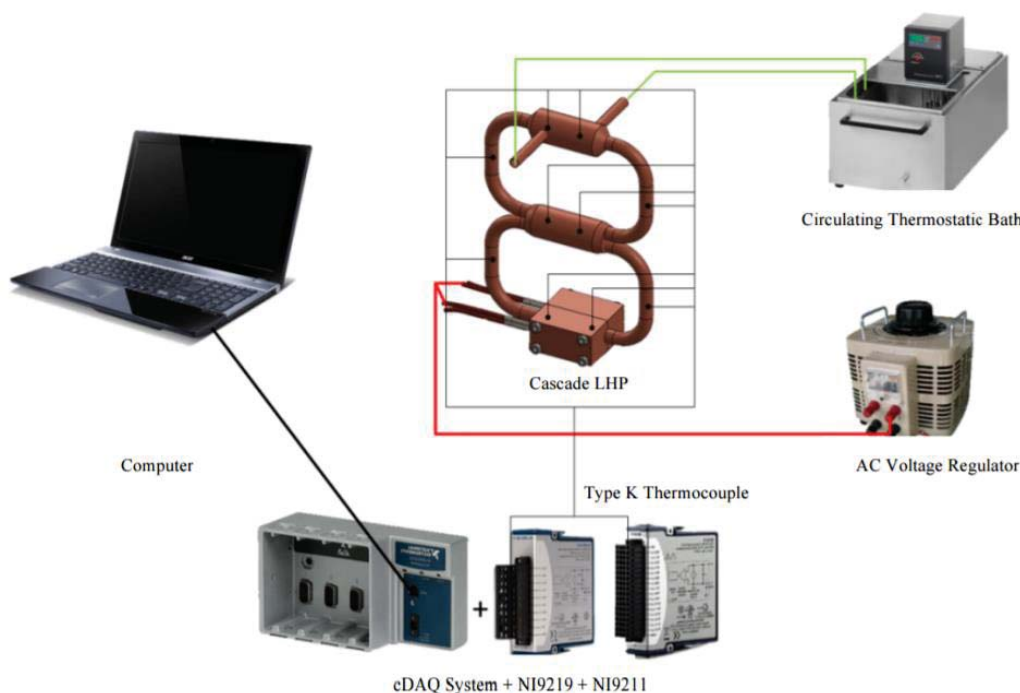
Fig. 3 Schematic Diagram of Experiment
