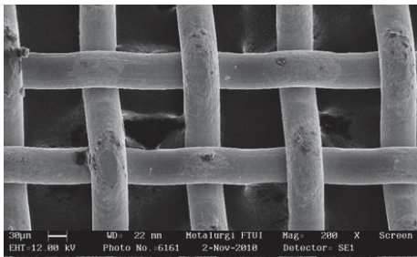
Fig. 6 SEM Visualization of Screen Mesh
