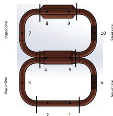
Fig. 2 Temperature Measurement Point of LHP
