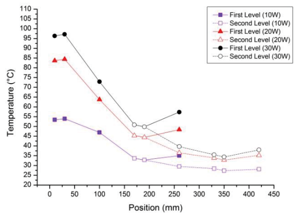
Fig. 7 Temperature Profile of Cascade LHP using Biomaterial
