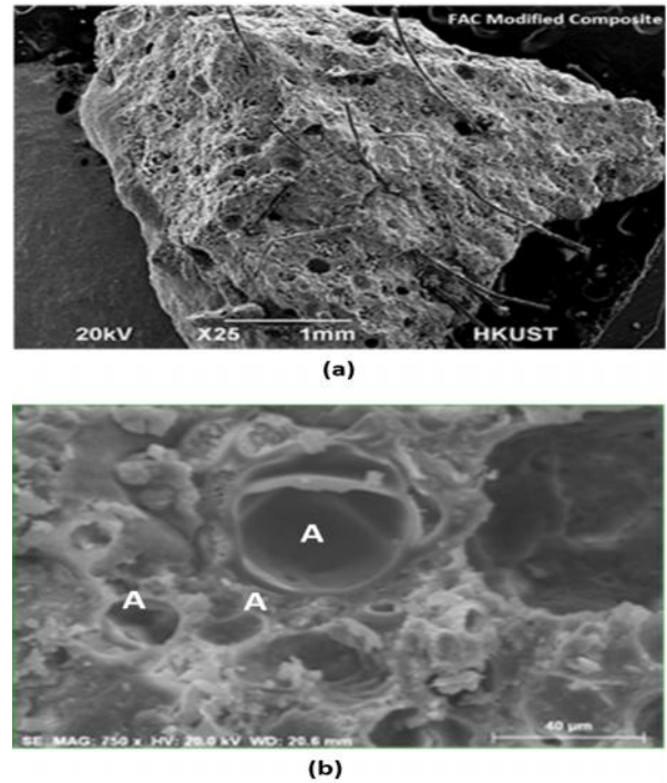
Fig. 8 (a) General morphology of the inner surface of FAC composites and (b) SEM image of FAC-aerogel specimen (aerogel particles are identified with the letter 'A')
