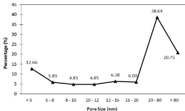
Fig. 2 Pore size distribution in aerogel particles
