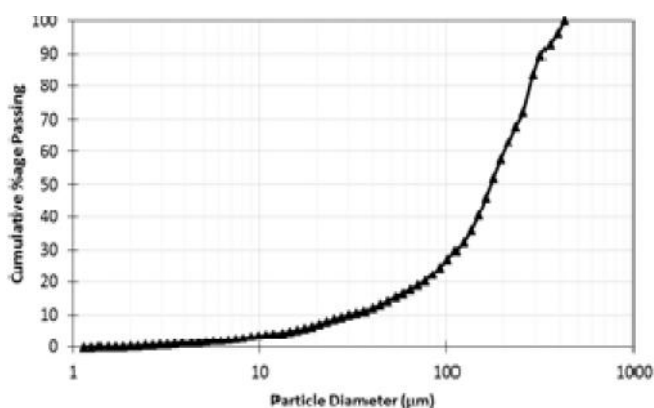
Fig. 1 Particle size distribution (by weight) of FACs
