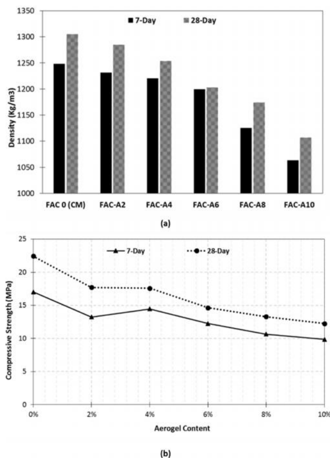
Fig. 5 (a) Density of FAC-Aerogel composites and (b) corresponding compressive strength
