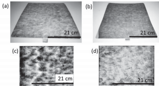
Fig. 7 Comparison of (a) calcium carbonate and (b) kaolin filled SMC plates and their corresponding transmitted light images (c) calcium carbonate filled SMC and (d) kaolin filled SMC with 53% mold coverage and 3 layers stacked below
