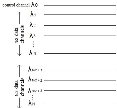
Fig. 1 Network architecture
