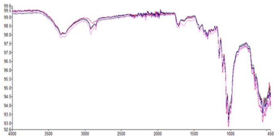
Fig. 11 FTIR spectra of sample 5 (20 % CD, 160°C, 5 min)
