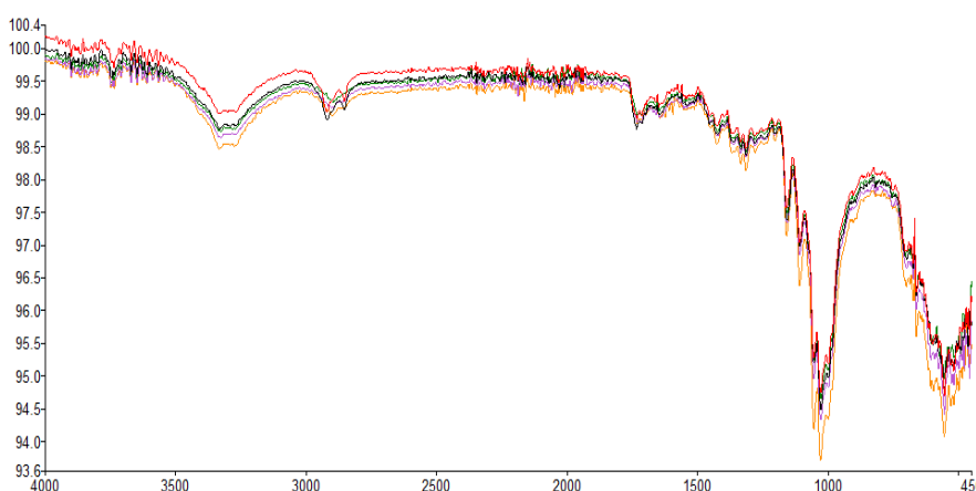
Fig. 18 FTIR spectra of sample 12 (25 % CD, 180°C, 10 min)
