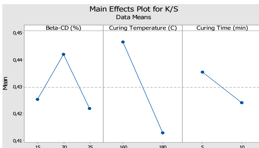
Fig. 34 Main effects plot for K/S
