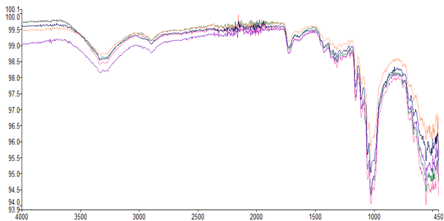
Fig. 14 FTIR spectra of sample 8 (20 % CD, 180°C, 10 min)
