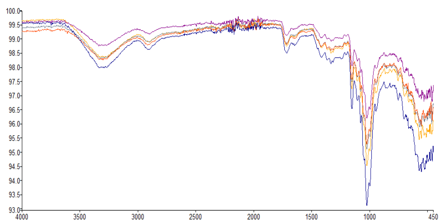
Fig. 15 FTIR spectra of sample 9 (25 % CD, 160°C, 5 min)
