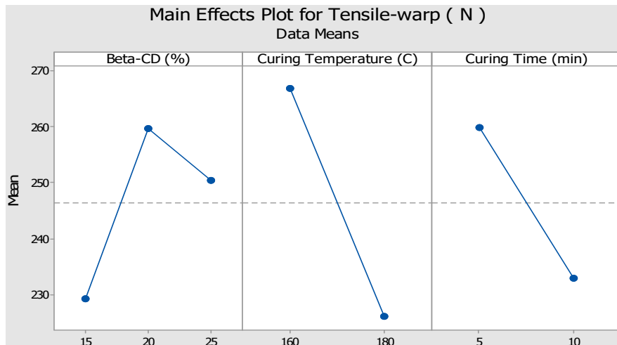
Fig. 30 Main effects plot for tensile strength of the warp yarns
