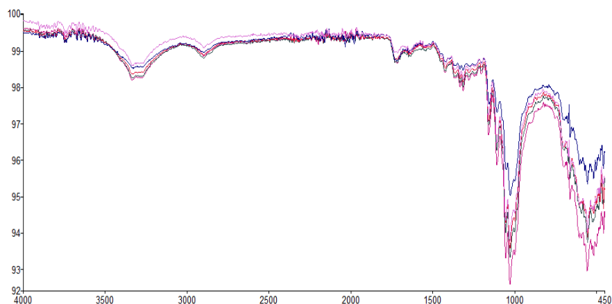
Fig. 17 FTIR spectra of sample 11 (25 % CD, 180°C, 5 min)
