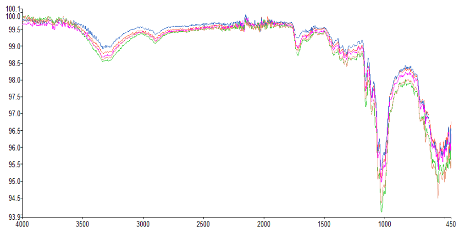
Fig. 16 FTIR spectra of sample 10 (25 % CD, 160°C, 10 min)
