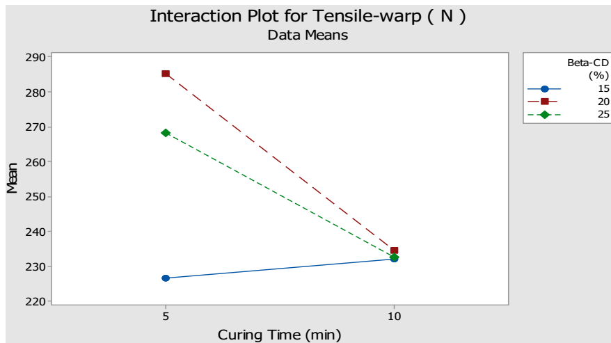
Fig. 32 Interaction plot for the change in tensile strength of the warp yarns according to curing time
