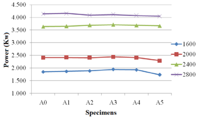
Fig. 5 Effect of the coated engine parts on the engine power
