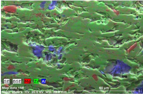
(a) SEM Coating Map
