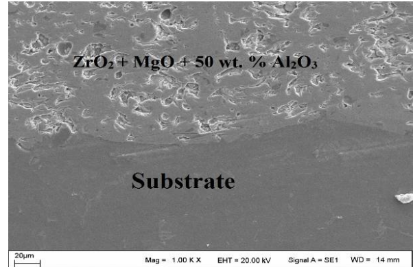
(b) SEM microscope view
