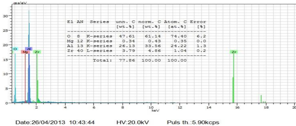
(c) EDS analysis
