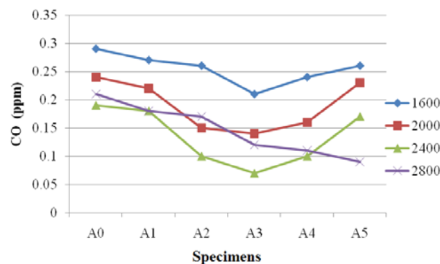
Fig. 9 Effect of the coated engine parts on the CO emissions
