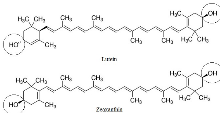
Fig. 3 Structural formulas of lutein and zeaxanthin [7]
