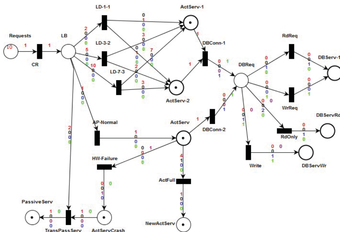
Fig. 4 CPN Model for Web Application Architecture
