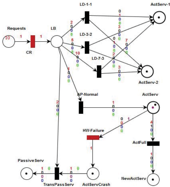
Fig. 2 Hardware Failure in Active-Passive mode
