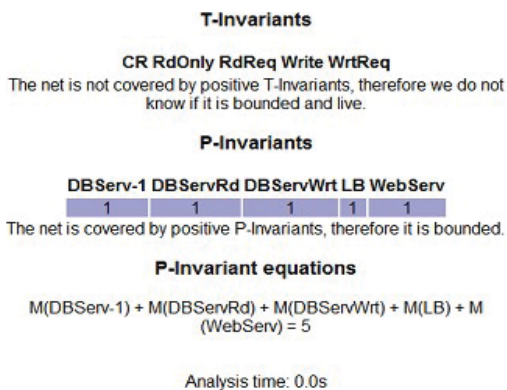
Fig. 9 Invariant analysis of DSS Model
