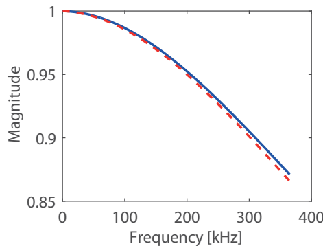
(b) Transmission coefficient
