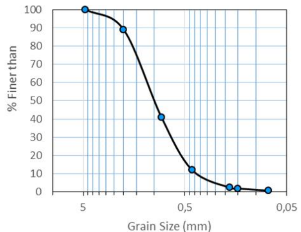
Fig. 1 Grain size distribution curve of the sand
