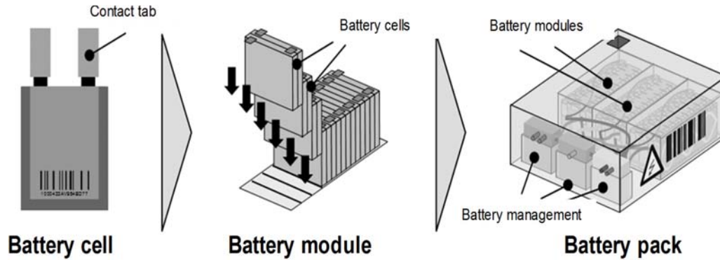
Fig. 1 From battery cells to a battery pack
