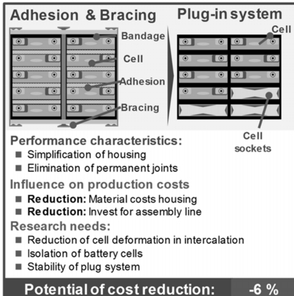
Fig. 4 Schematic presentation of a plug-in system [36]
