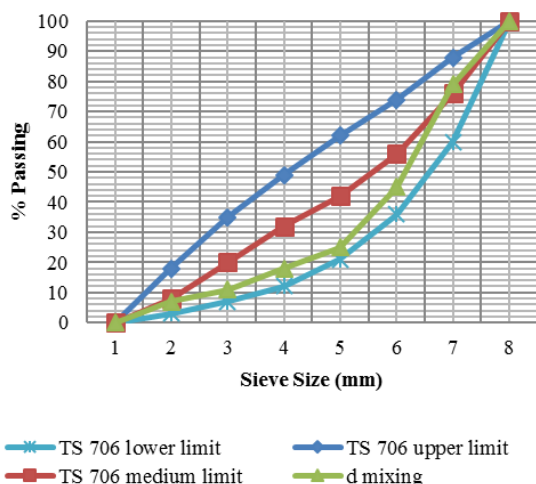
Fig. 1 Grading curve of aggregate
