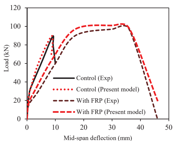
Fig. 4 Load-deflection curves for composite strengthened beams
