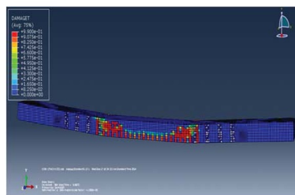
Fig. 3 Crack paths by ABAQUS software with FRP and without FRP sheets
