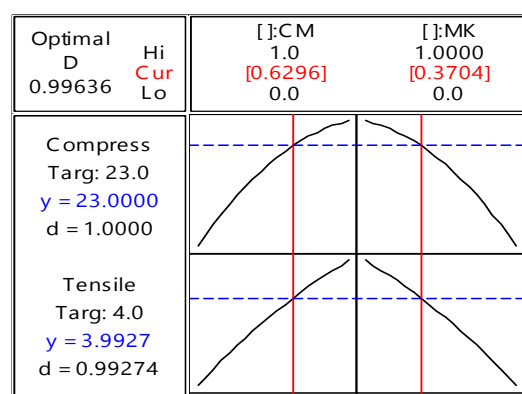
Fig. 1 Optimal proportion of Udon Thani metakaolin
