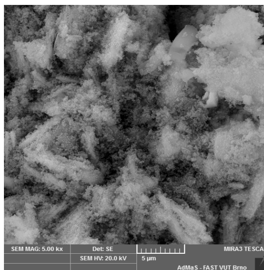
Fig. 8 SEM photos (5000× magnification) of REF geopolymer mortar
