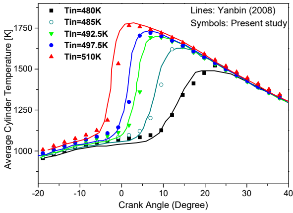
Fig. 4 Comparison between the present study and Yanbin's result [15]
