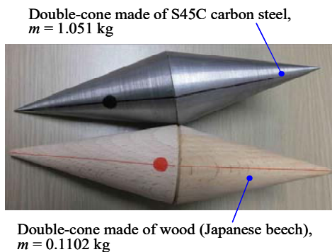
Fig. 1 Photographs of the tested metallic and wooden double-cones
