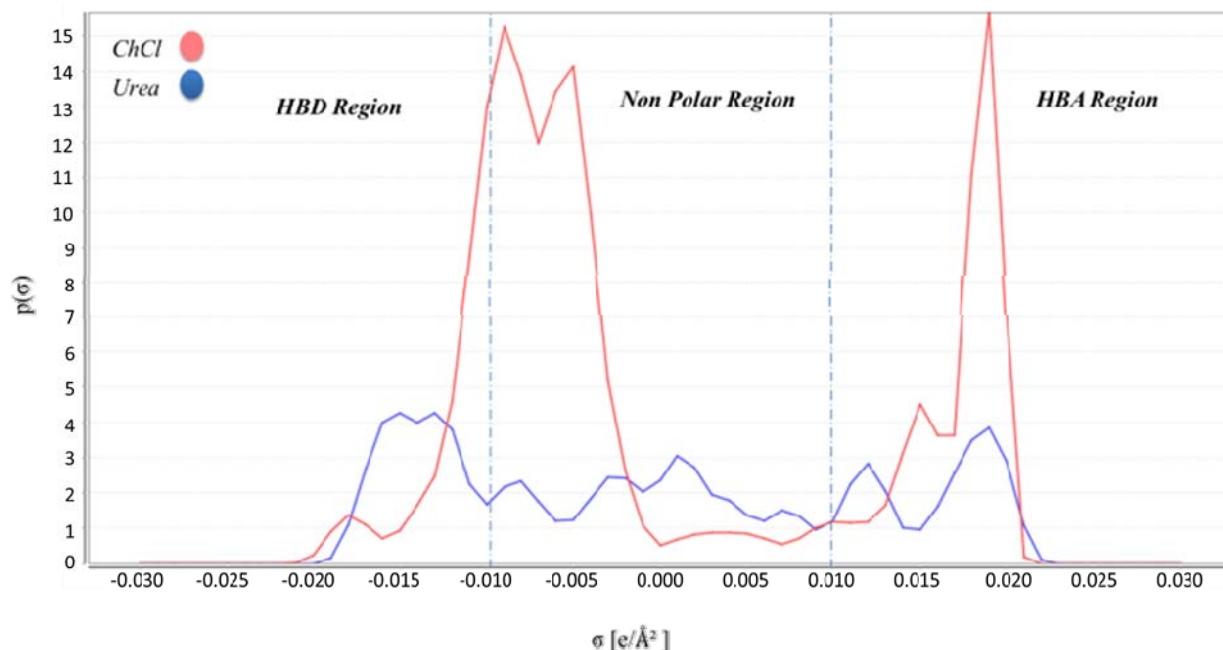
Fig. 2 \sigma profile of ChCl, Urea
