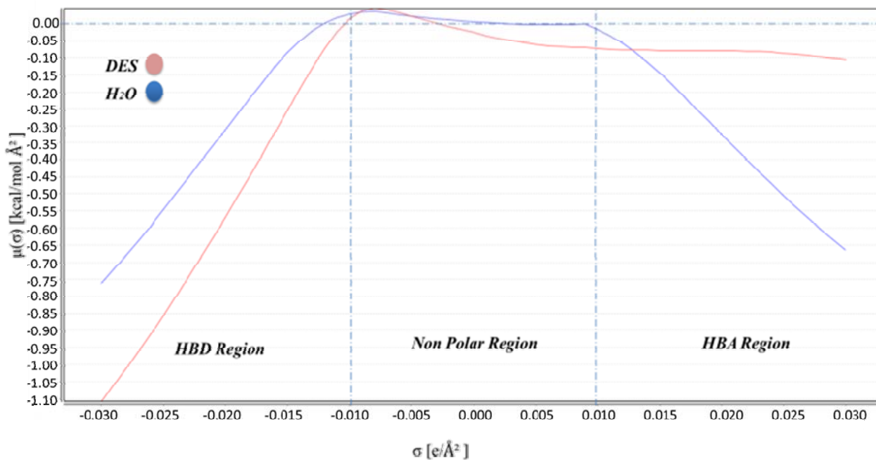
Fig. 3 \sigma potential of DES and water
