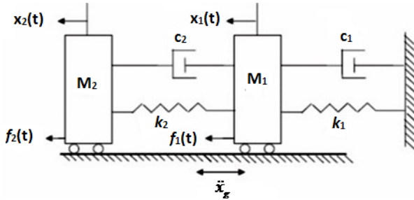
Fig. 2 Proposed 2-DOF Model
