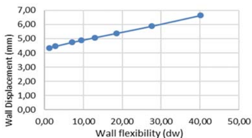
Fig. 6 Effect of wall flexibility on wall displacement
