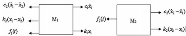
Fig. 3 Free-Body Diagram of Wall and Backfill-soil
