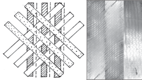
(a) Preform Sample
