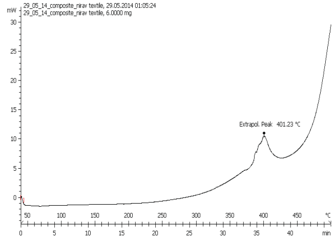
Fig. 6 DSC Analysis of Glass Laminate (GM0°/±45°)
