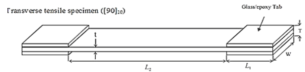
L1=Jaw Length=50mm, L2=Gauge Length=150mm T=Thickness, W=Width=25mm
