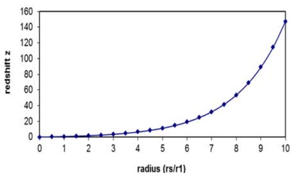
Fig. 2 The calculated gravitational redshift from (9)
