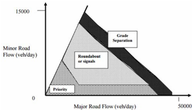
Fig. 4 Flow ranges by intersection type [6]
