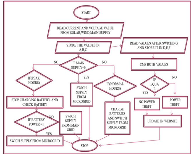
Fig. 2 Scheduling flowchart
