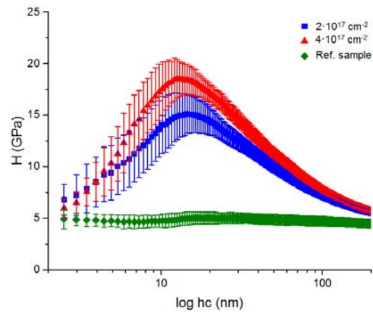
Fig. 4 Depth profiles of indentation hardness
