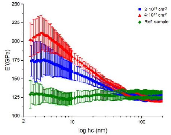
Fig. 3 Depth profiles of reduced storage moduli
