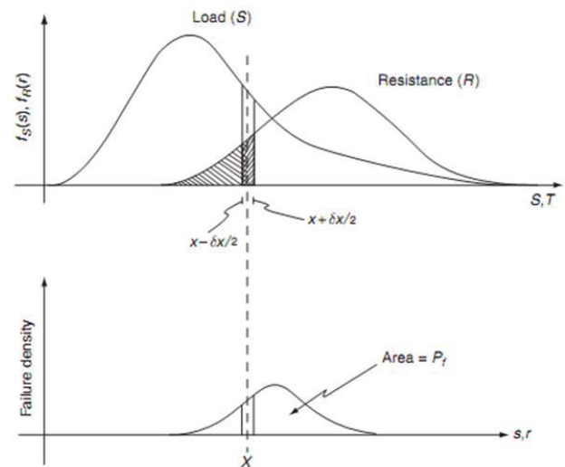
Fig. 1 Diagram explaining the probability of failure [3]
