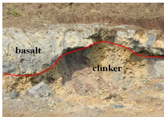
Fig. 5 Clinker layer exposed in a testing area
