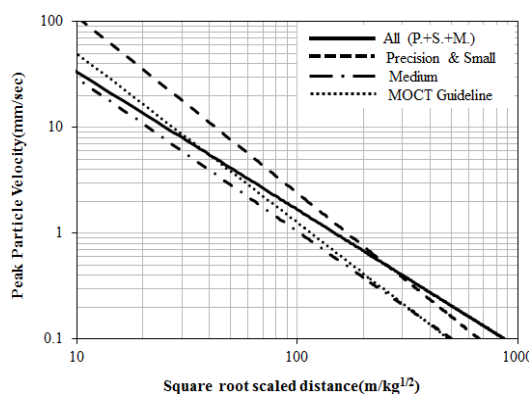
Fig. 10 Comparison of blasting vibration characteristics
