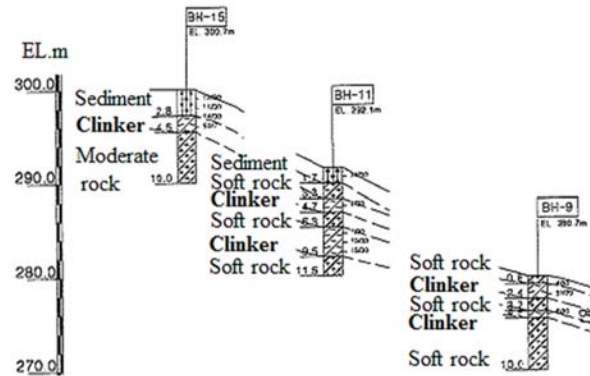
Fig. 6 Geological profile
