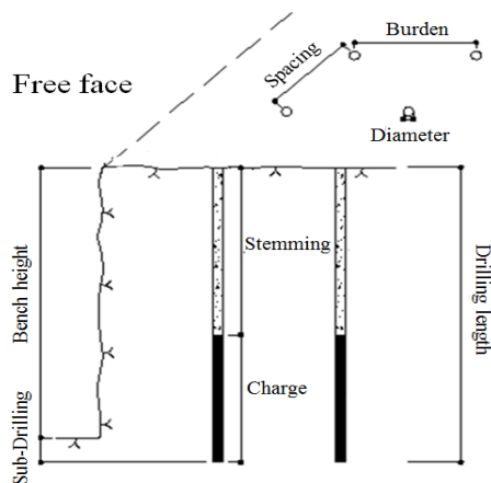
Fig. 7 Schematic diagram of blasting pattern
