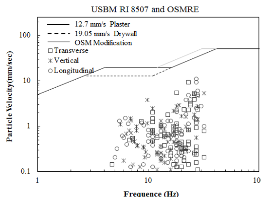
Fig. 11 Analysis of vibrations frequency
