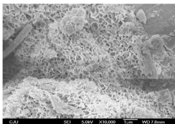
Fig. 2 FE-SEM observation ( \times 10,000 )
