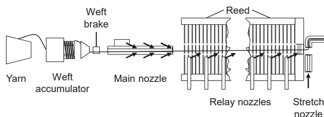
Fig. 1 Schematic view of air-jet weft insertion system
