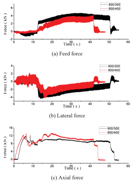
Fig. 2 Force curves under different feed speeds of tool
