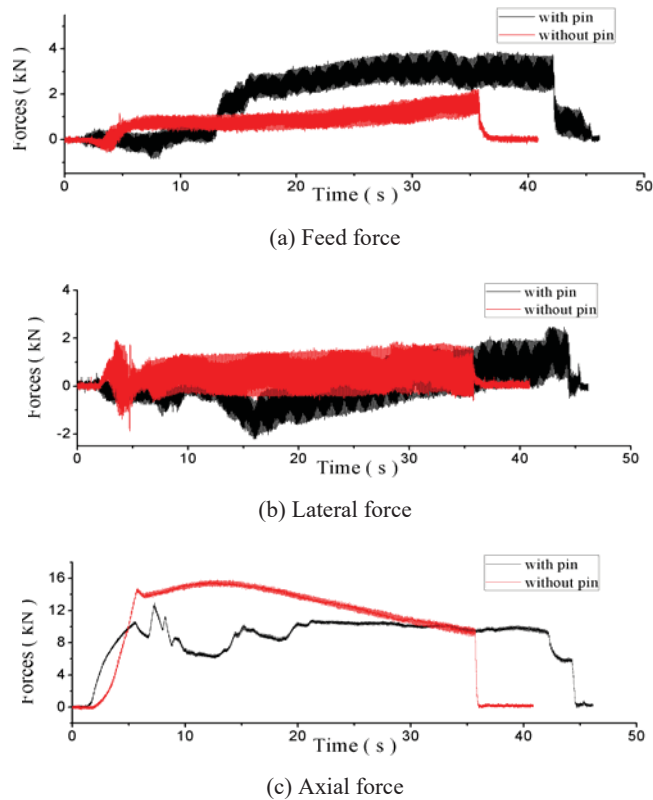
Fig. 5 The effect of pin for forces
