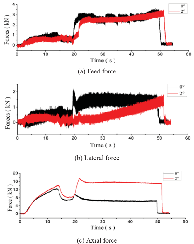
Fig. 4 Force curves under different tilt angles
