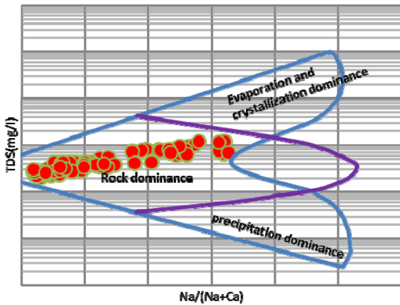
Fig. 13 Gibbs diagram for the Qare Sou Catchment
