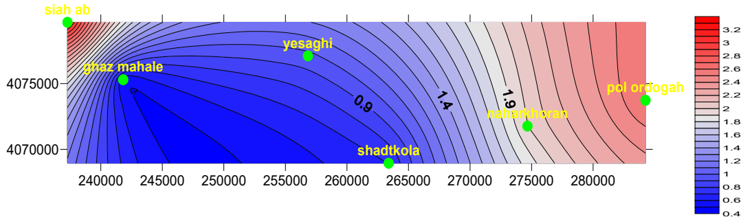
Fig. 11 distribution of Sulfate in Qare-Sou
