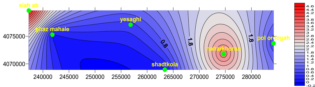
Fig. 12 Distribution of sodium in Qare-Sou
