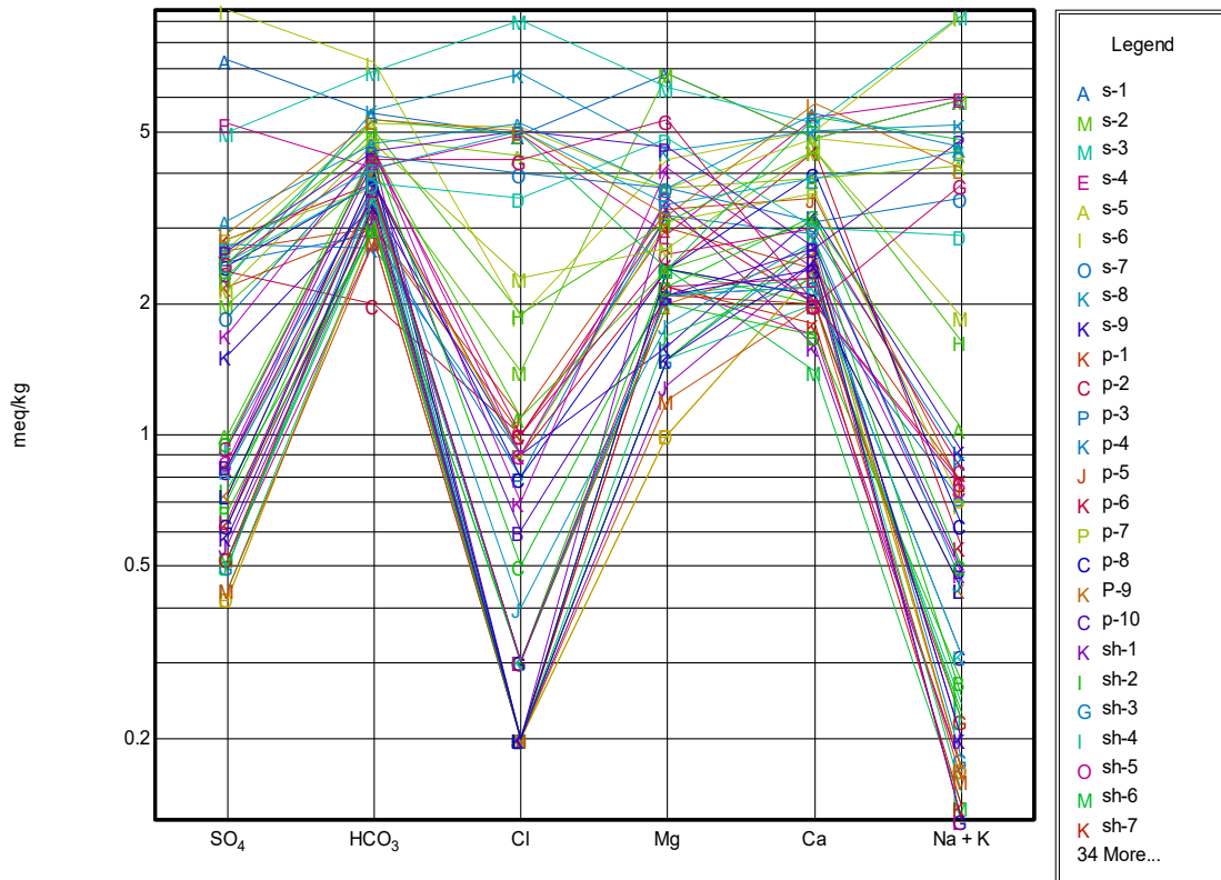
Fig. 16 Schoeller diagram of Qare-sou catchment
