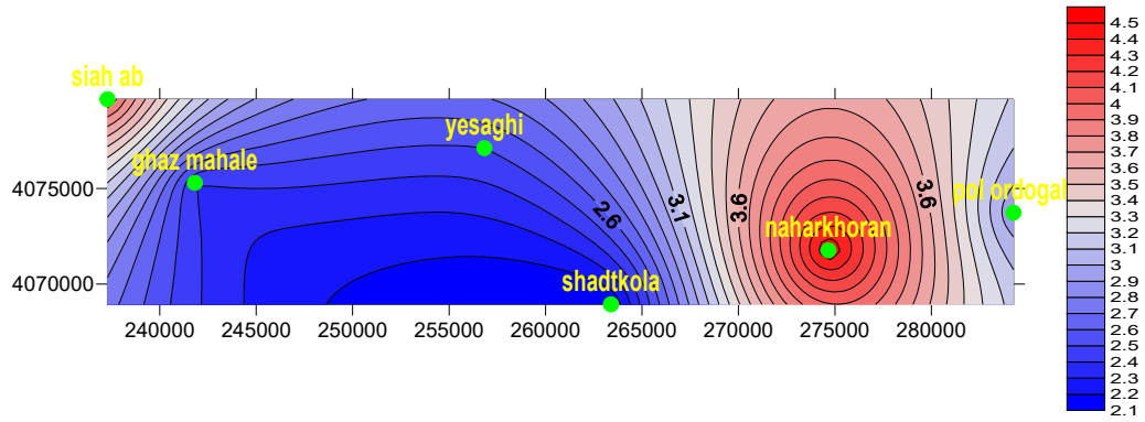
Fig. 6 Distribution of Calcium in Qare-Sou
