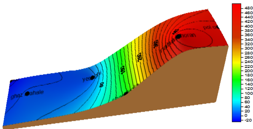
Fig. 4 Topography of sampling stations
