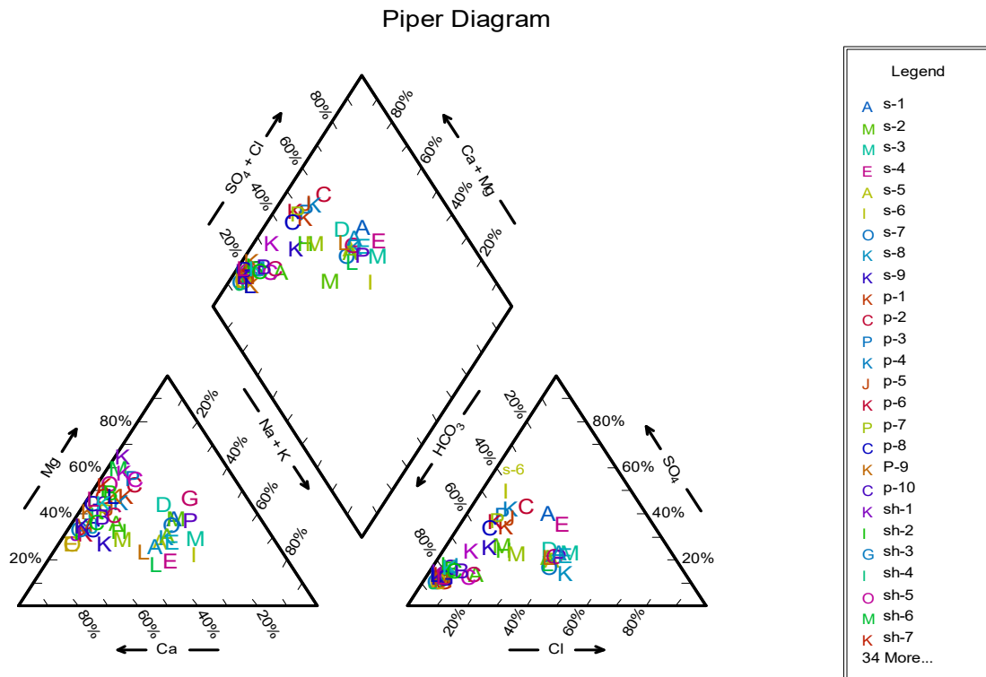
Fig. 14 Piper diagram of Qare-sou catchment.
