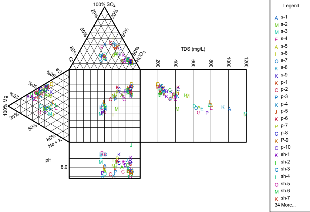
Fig. 15 Durov diagram of Qare-sou catchment
