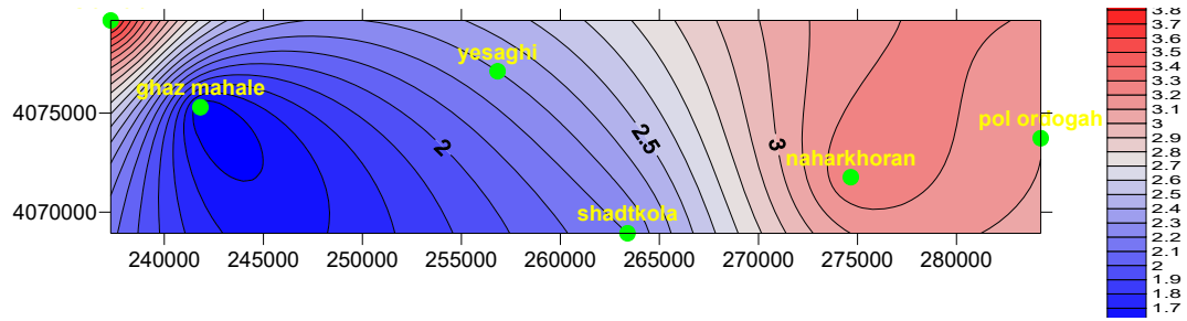
Fig. 10 Distribution of Magnesium in Qare-Sou
