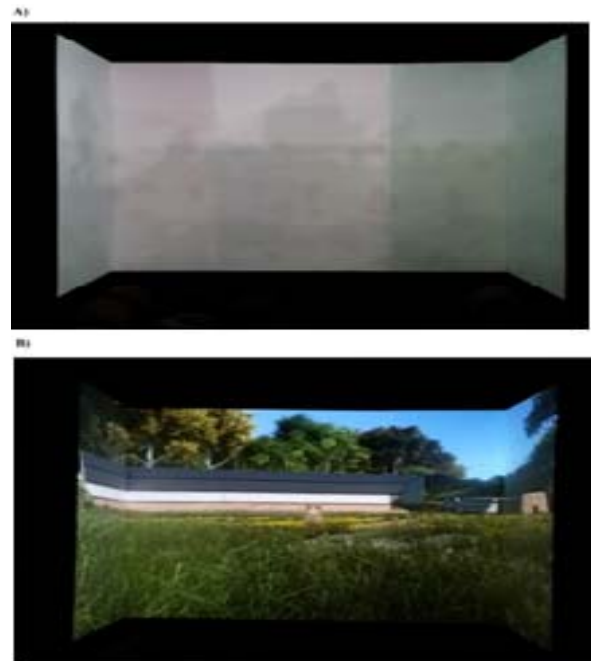
Fig. 8 The result of implemented photometric recalibration algorithm (A) Before use, (B) after use
