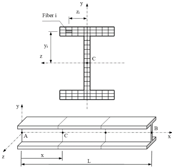
Fig. 1 Discretization of beam-column element
