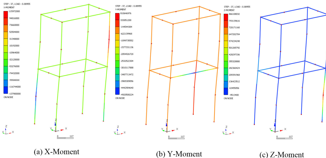
Fig. 12 Nodal reaction moments of two-story space steel frame using fiber-hinge beam-column element at the ultimate load factor
