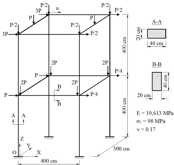
Fig. 8 Two-story space steel frame
