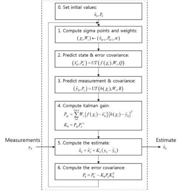
Fig. 2 UKF Algorithm
