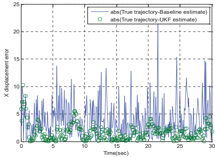
Fig. 9 Localization errors (x displacement)
