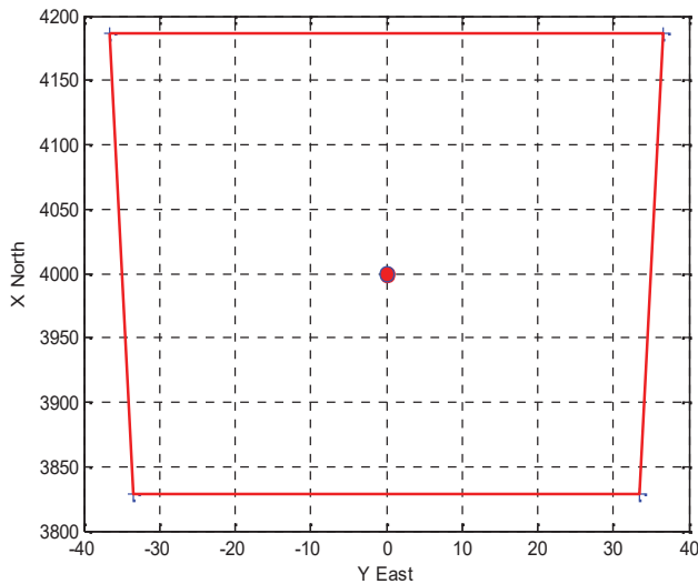
Fig. 4 Area imaged by the camera: high altitude
