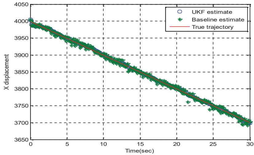
Fig. 7 UKF results (x displacement)
