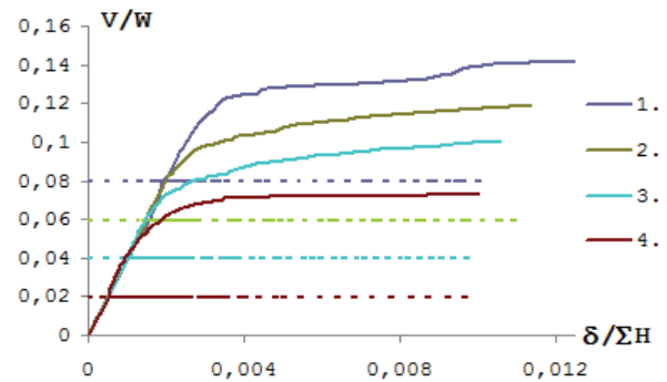
Fig. 11. Load-Displacement Curves for 6-story buildings for Z3
