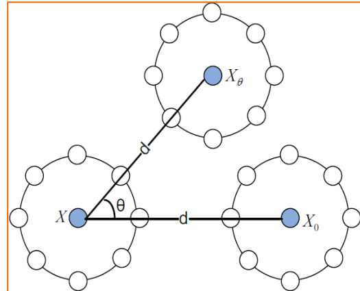
Fig. 7 Co-occurrence Model
