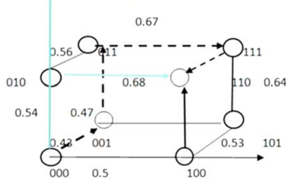
Fig. 4 Hypercube Model
