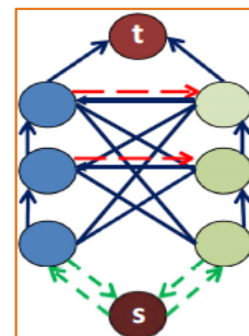
Fig. 5 Routing Model
