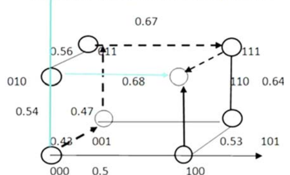
Fig. 4 Hypercube Model
