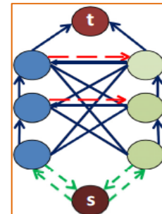
Fig. 5 Routing Model
