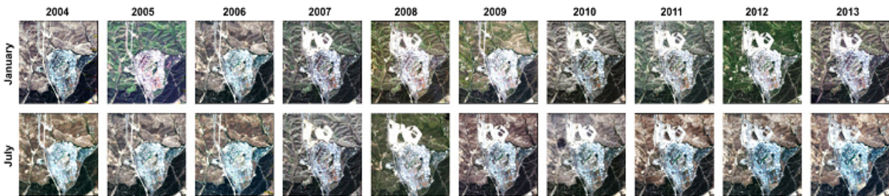
Fig. 3 Landsat time series images from 2004 to 2013
