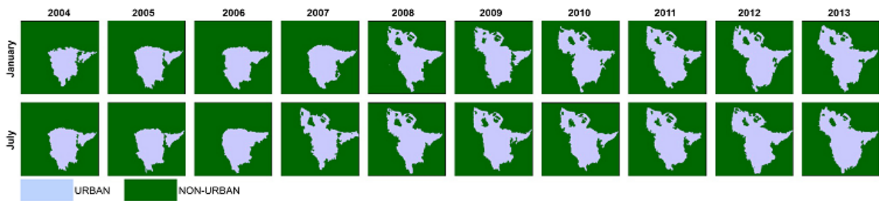
Fig. 4 Obtained classification
