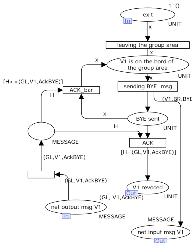
Fig. 10 Departure Petri Net
