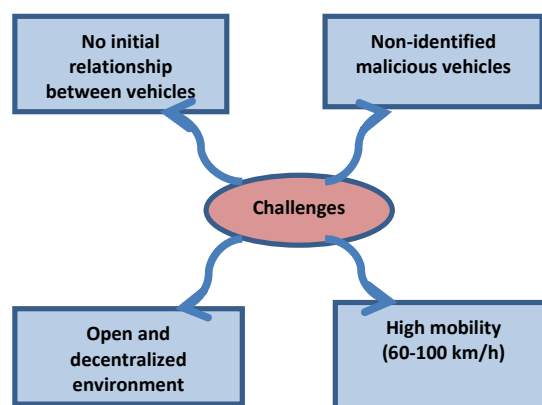
Fig. 1 VANET challenges
