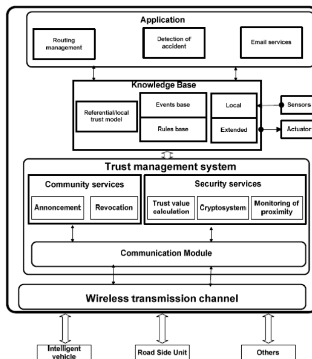
Fig. 5 Functional model of the application
