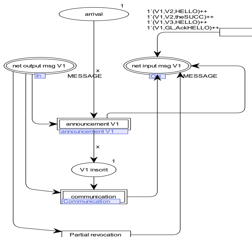
Fig. 6 Model of an Active vehicle
