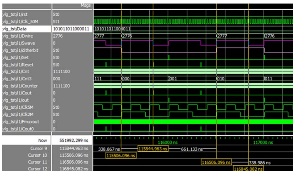
Fig. 3 Simulation results using Modelsim
