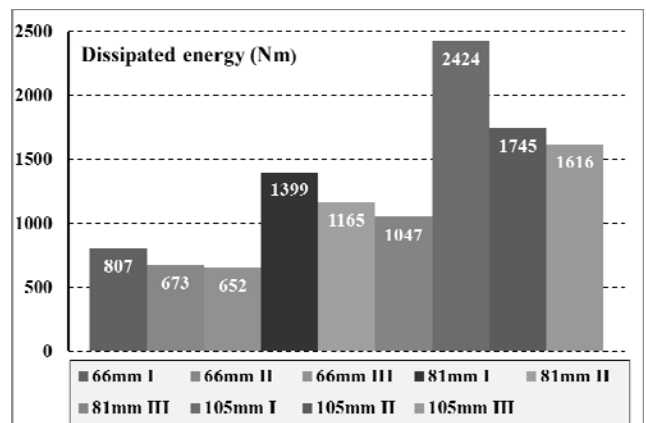
Fig. 13 Dissipated energy during the seismic type test
