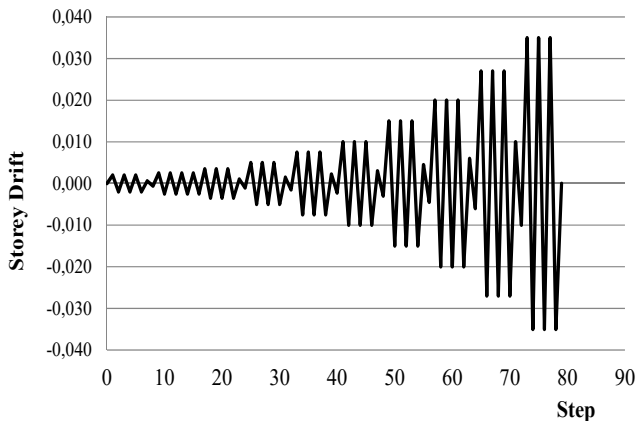
Fig. 8 Loading history
