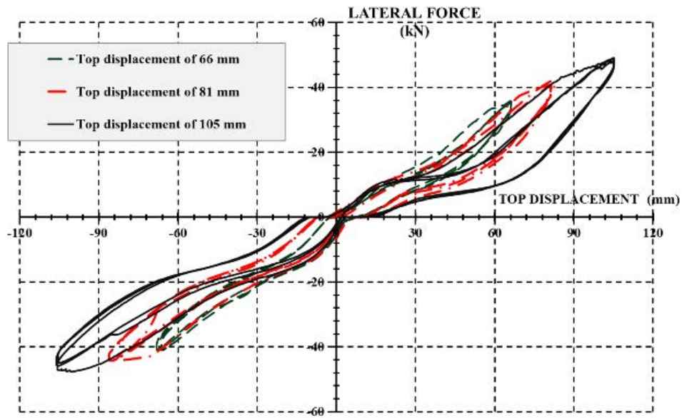
Fig. 9 Lateral load - Top displacement
