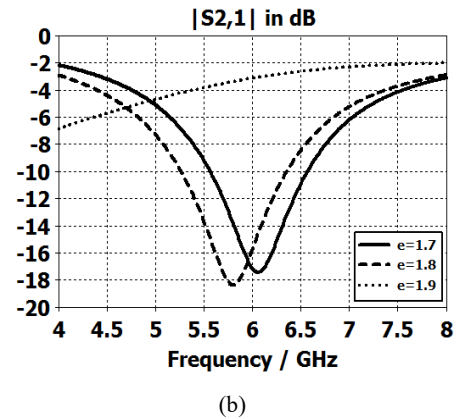
Fig. 7 Simulation of S11 (a) and S21 (b) with varied parameter e
