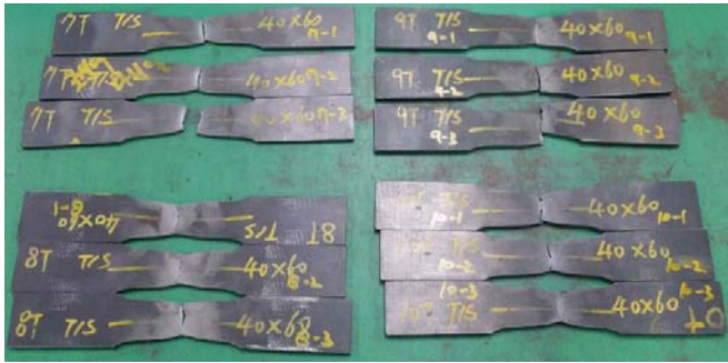
Fig. 3 Fracture of tension coupon test result
