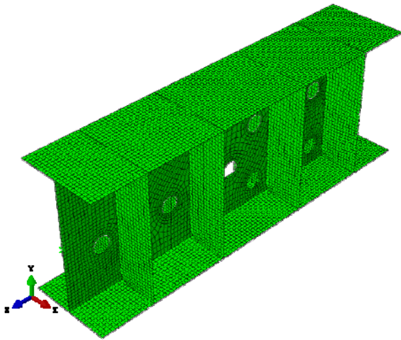
Fig. 4 3D meshed analysis model
