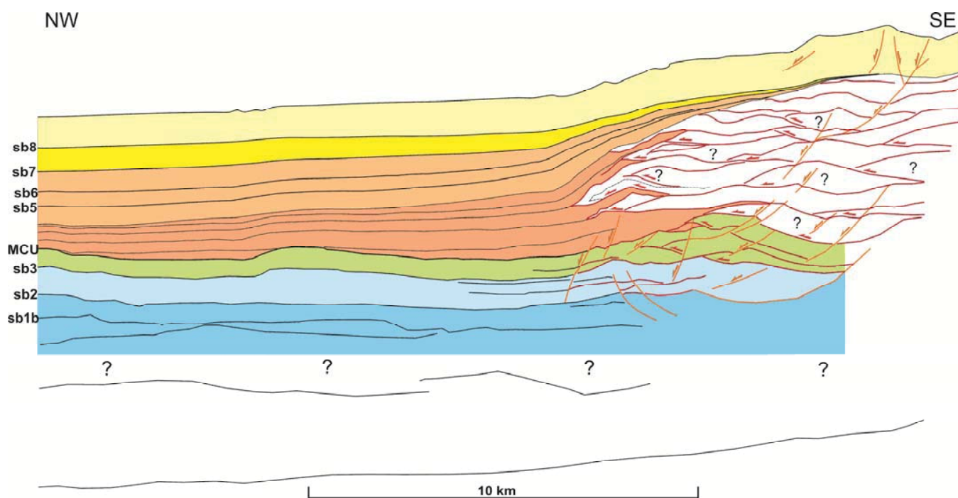
Fig. 2 Internal structure of the fold-and-thrust belt, Cuba
