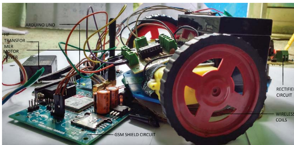
Fig. 7 GSM controlled robot
