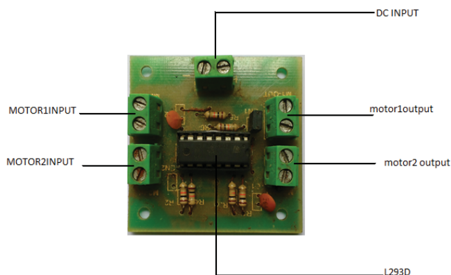
Fig. 4 Motor driver circuit
