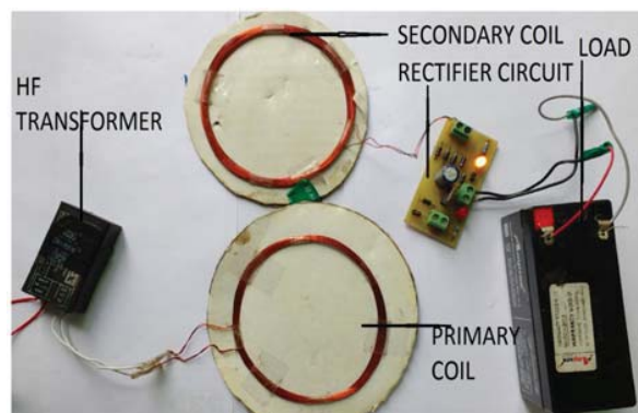
Fig. 2 Circuit connection of wireless power transfer
