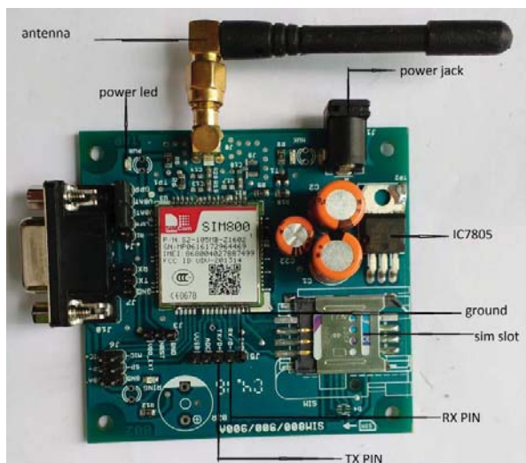
Fig. 5 GSM shield circuit configuration
