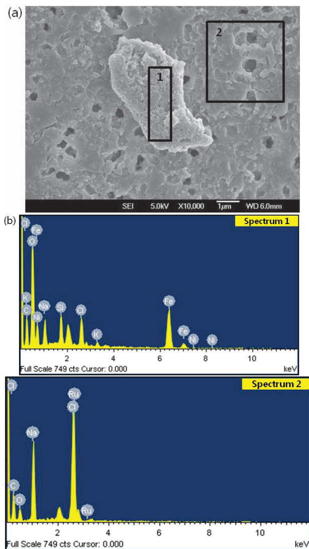
Fig. 4 (a) SEM image of E. coli O157:H7 cell bound with MNP-Apts, (b) EDS pattern of the cell surface with MNP-Apts (spectrum 1) and the membrane surface (spectrum 2)
