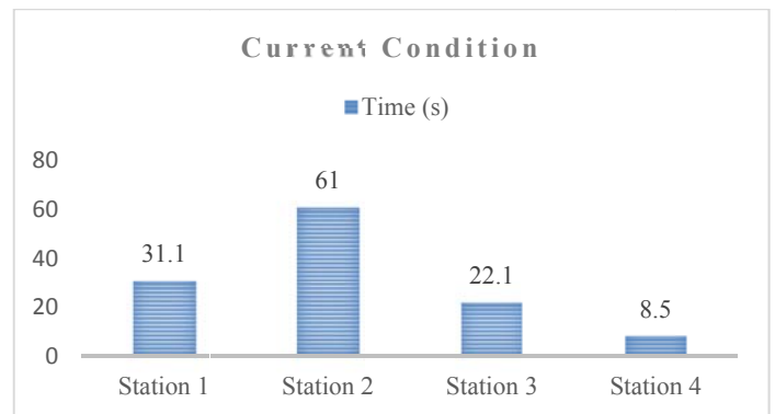
Fig. 3 Cycle time in each station before improvement
