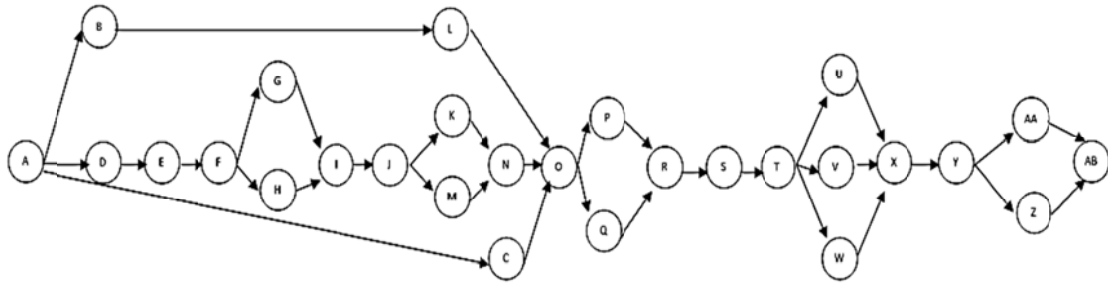
Fig. 4 Precedence diagram of piston assembly line
