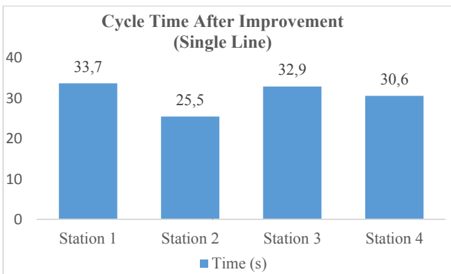
Fig. 6 Cycle time for each workstation after improvement
