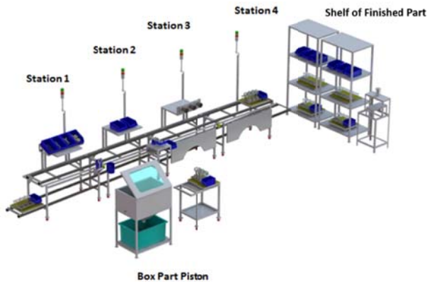
Fig. 1 Piston assembly line in manufacturing system laboratory
