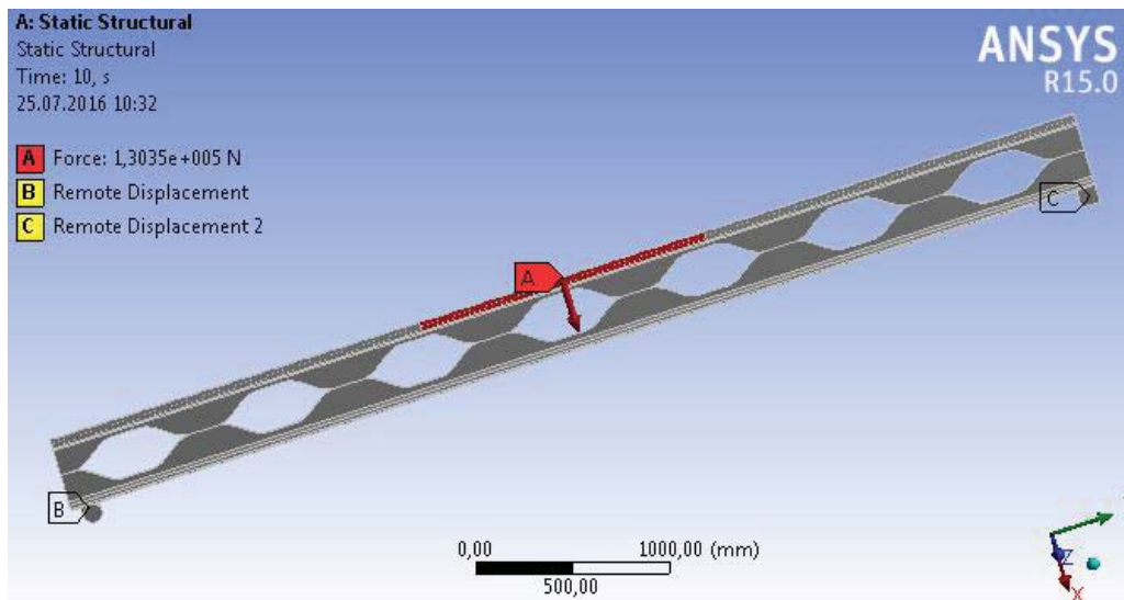
Fig. 10 Static structure of NPI_SB_240 Angelina™ beam
