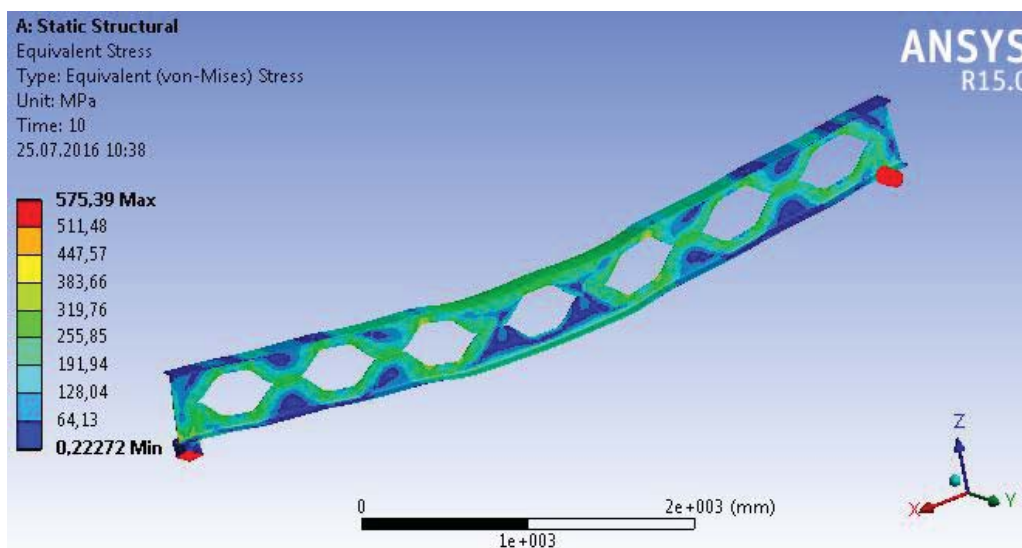
Fig. 19 Equivalent stress of NPI_SB_300 Angelina™ beam
