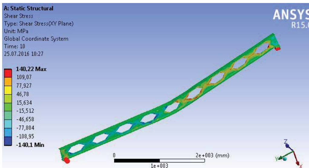
Fig. 8 Shear stress of NPI_SB_200 Angelina™ beam
