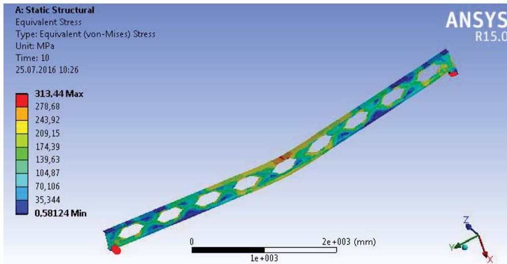
Fig. 7 Equivalent stress of NPI_SB_200 Angelina™ beam
