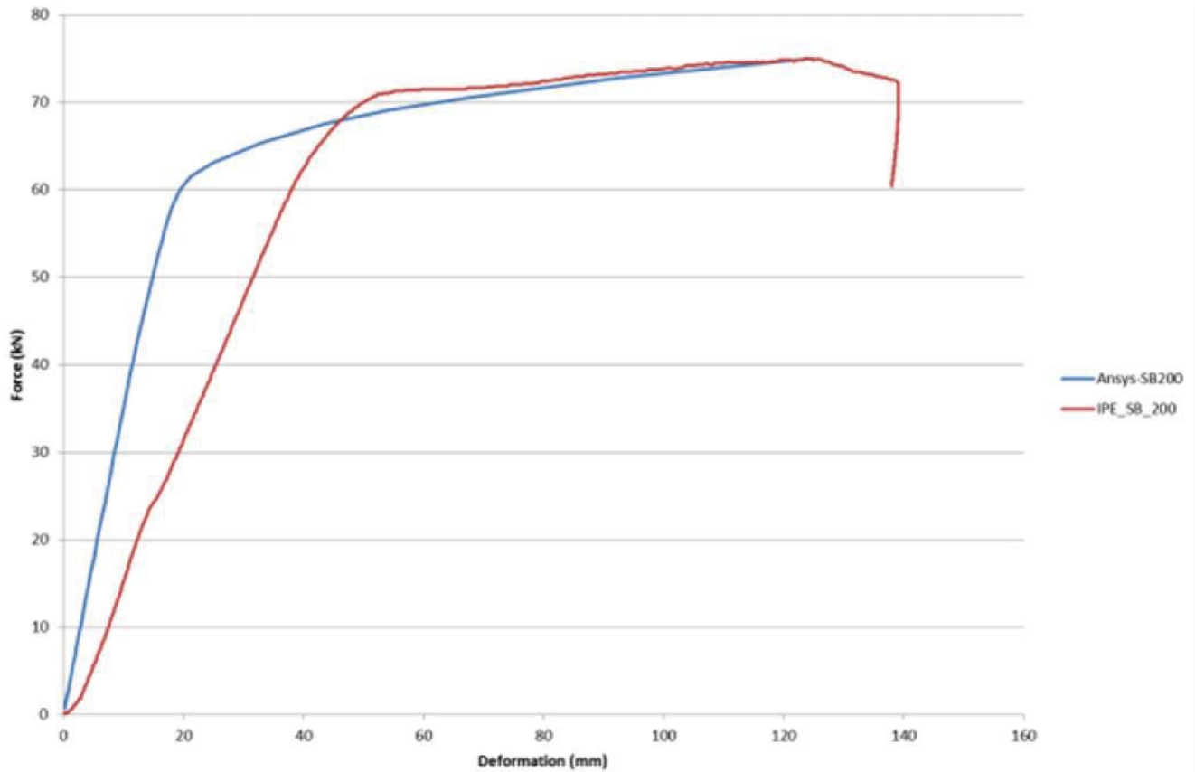
Fig. 9 Load-displacement curve of NPI_SB_200 Angelina™ beam
