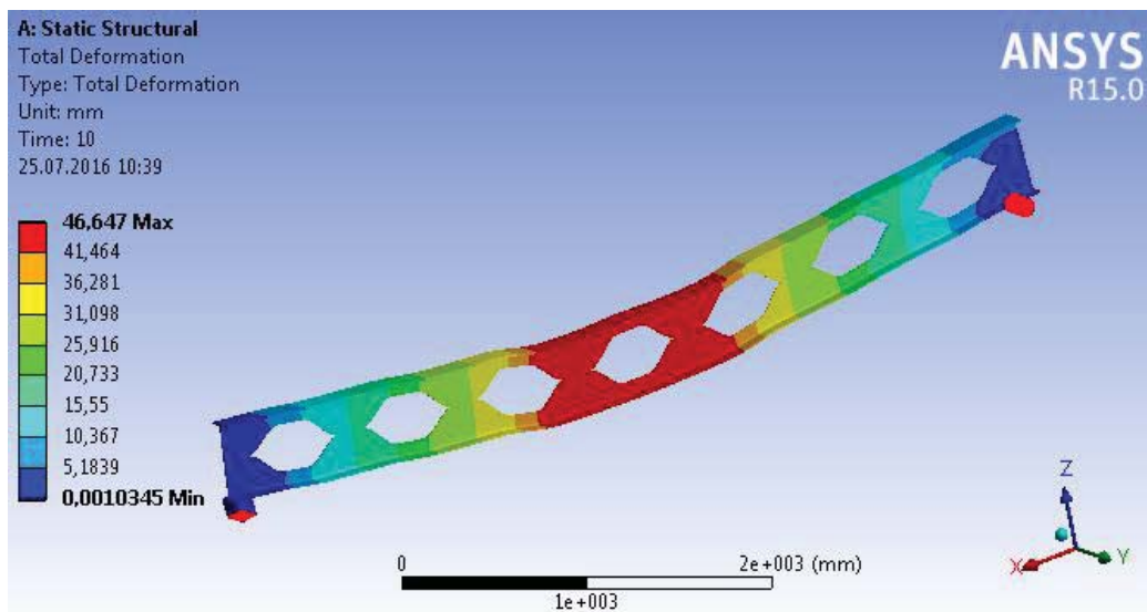
Fig. 18 Total deformation of NPI_SB_300 Angelina™ beam
