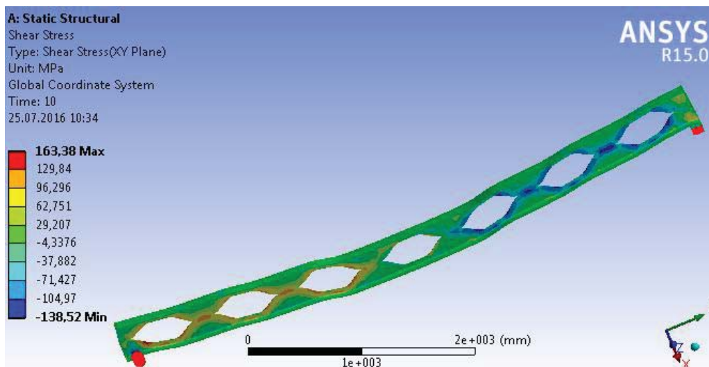
Fig. 14 Shear stress of NPI_SB_240 Angelina™ beam
