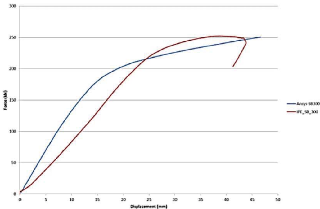
Fig. 21 Load-displacement curve of NPI_SB_300 Angelina™ beam
