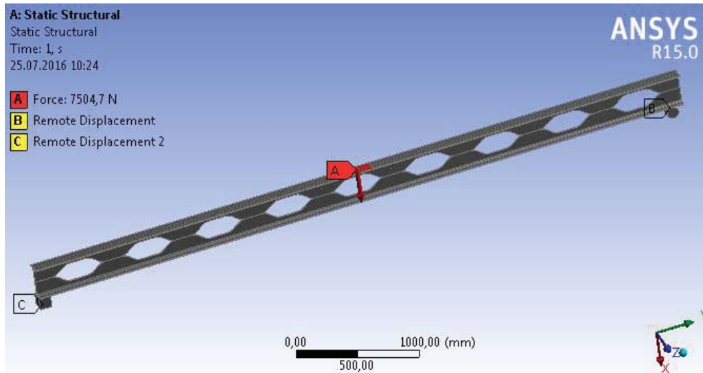
Fig. 4 Static structure of NPI_SB_200 Angelina™ beam
