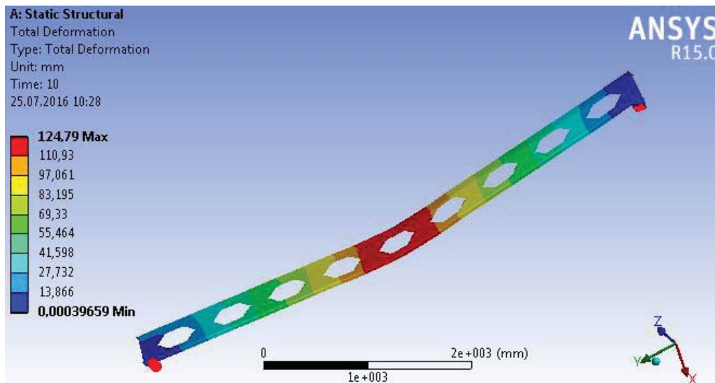
Fig. 6 Total deformation of NPI_SB_200 Angelina™ beam
