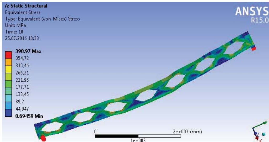
Fig. 13 Equivalent stress of NPI_SB_240 Angelina™ beam
