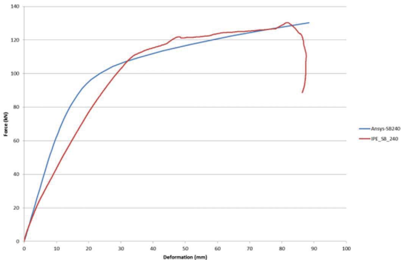
Fig. 15 Load-displacement curve of NPI_SB_240 Angelina™ beam
