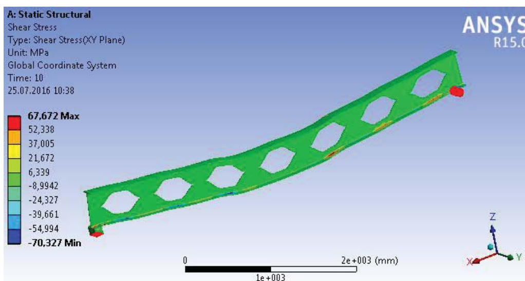
Fig. 20 Shear stress of NPI_SB_300 Angelina™ beam
