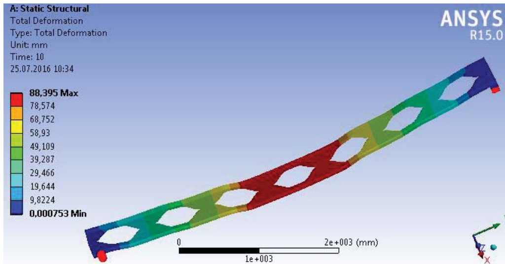
Fig. 12 Total deformation of NPI_SB_240 Angelina™ beam
