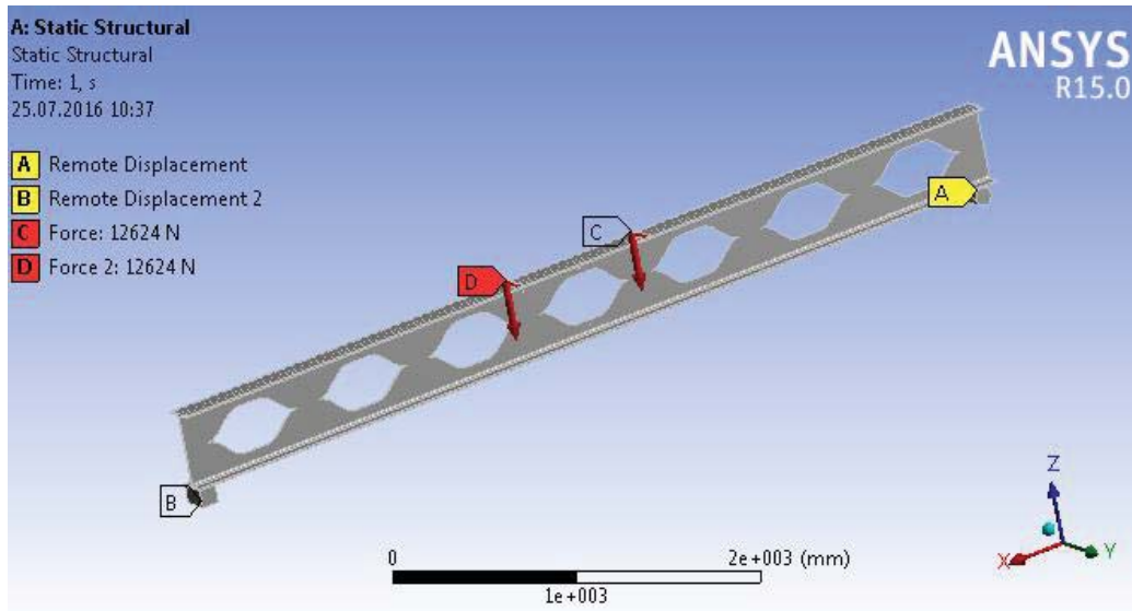
Fig. 16 Static structure of NPI_SB_300 Angelina™ beam
