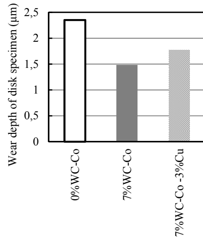
Fig. 8 Wear depth of sintered disk specimens
