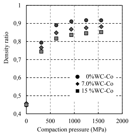
Fig. 5 Relationship between compaction pressure and density ratio
