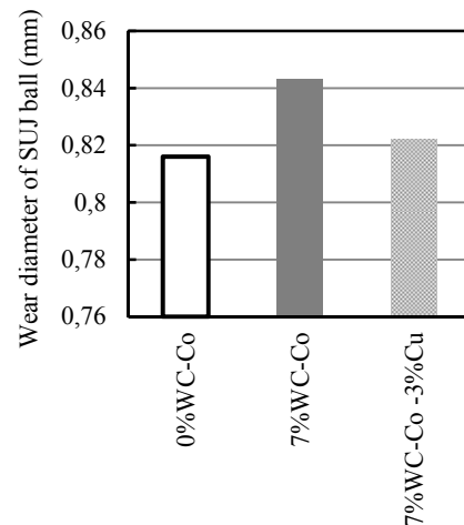
Fig. 9 Diameter of wear mark on counter ball
